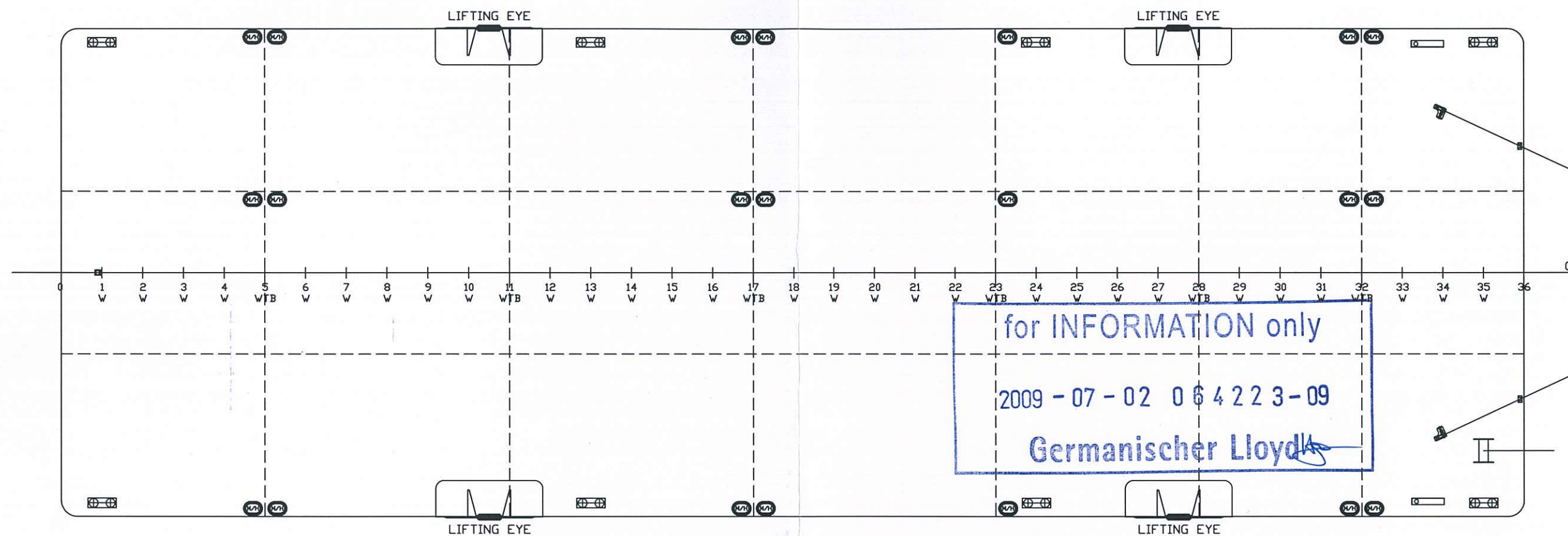
MAIN DECK
