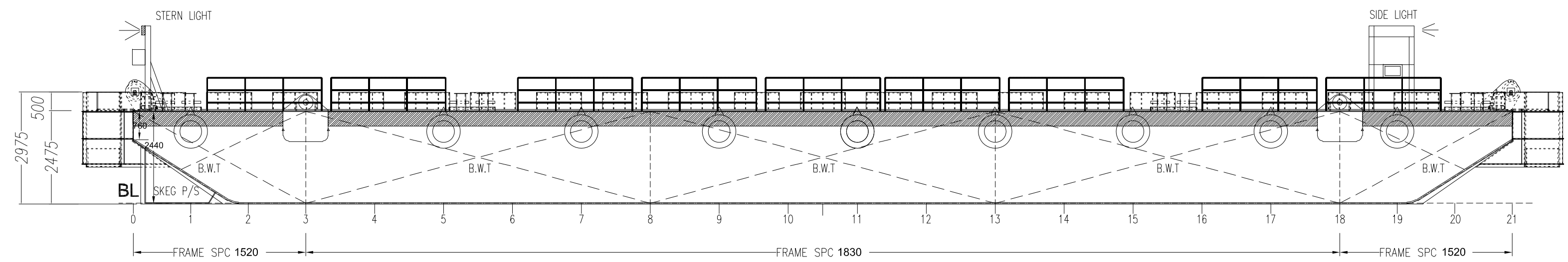
OUTBOARD PROFILE
