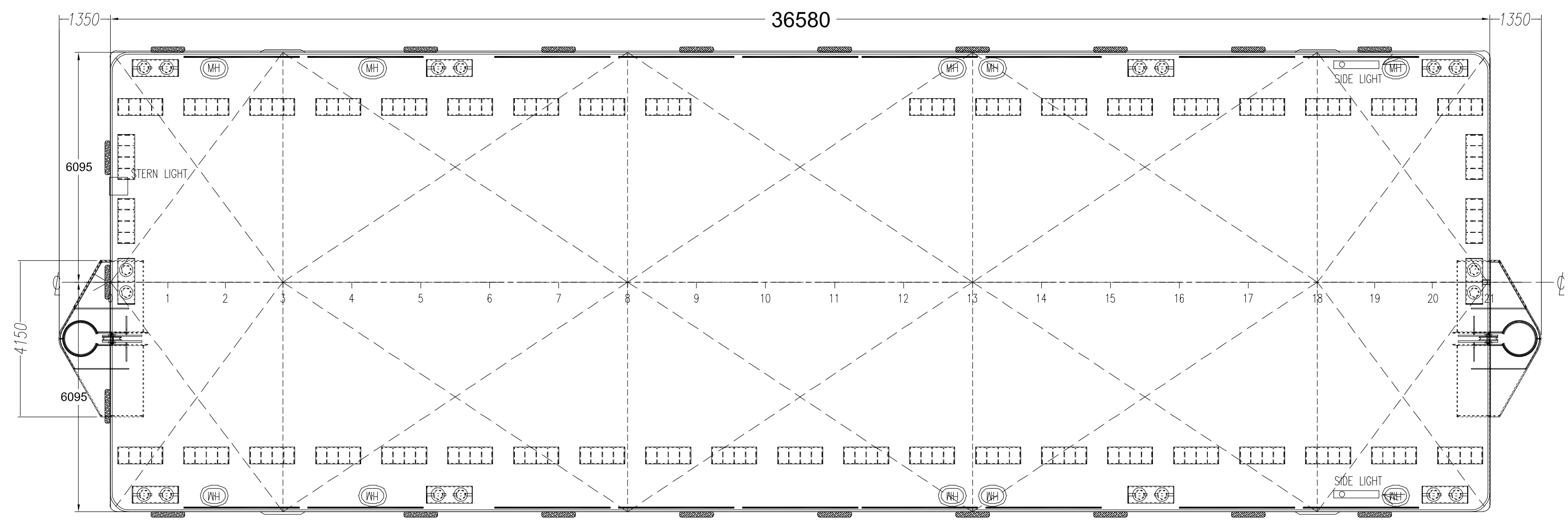
MAIN DECK
