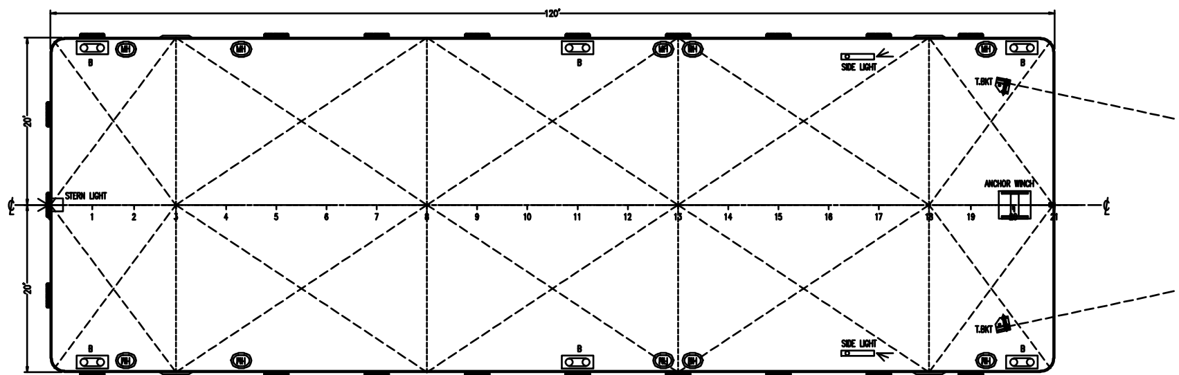
MAIN DECK
